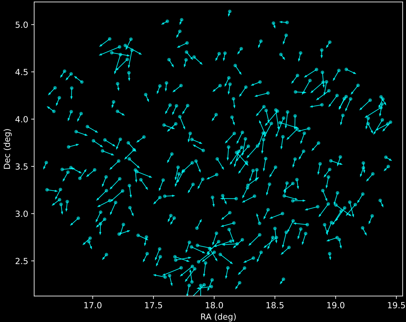
APOGEE DR17 Noise Stream Proper Motion Vectors (n=276)
