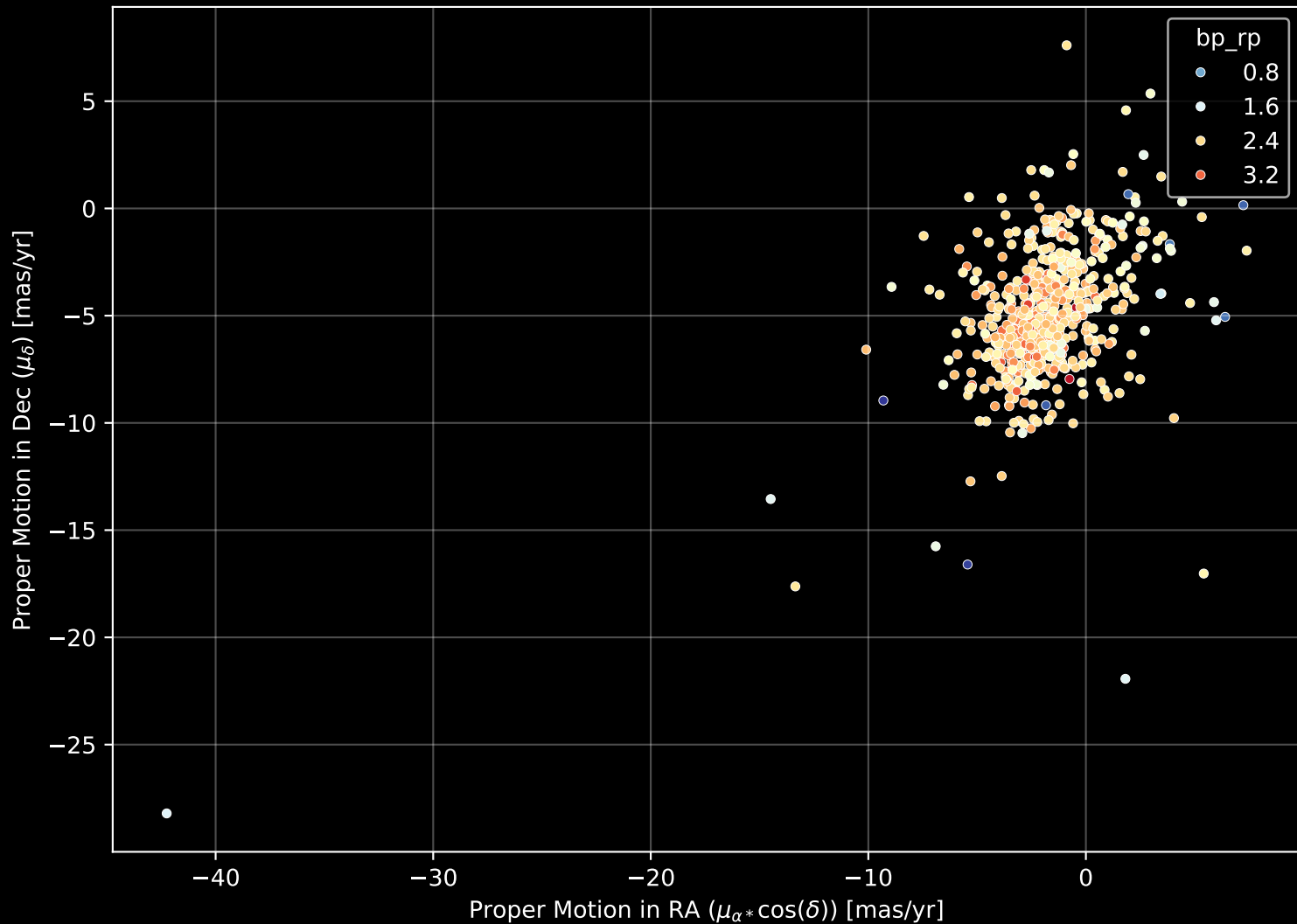
APOGEE DR17 Field: [034+06] Proper Motion Diagram (n= 608)
