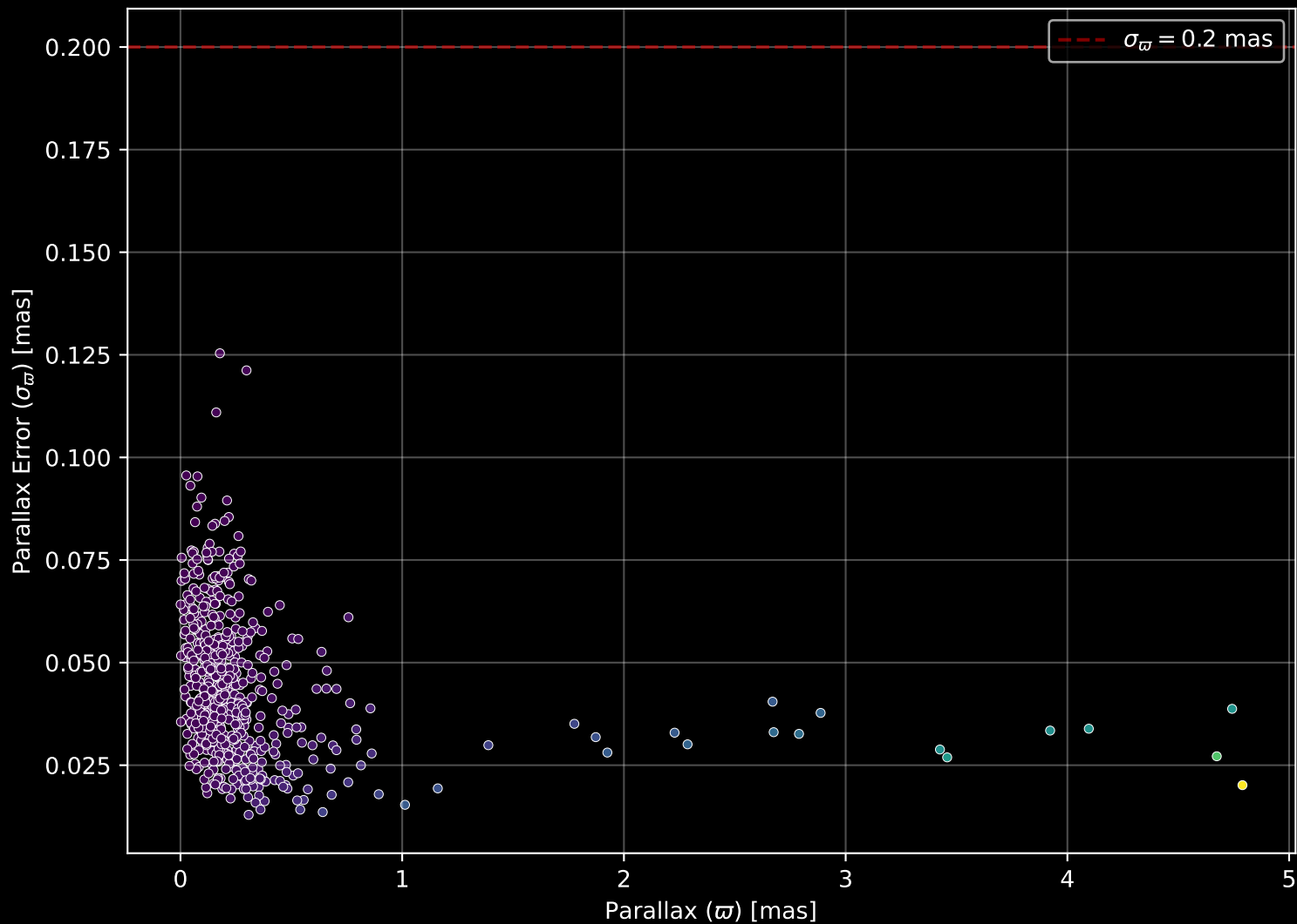
APOGEE DR17 Field: [034+06] Parallax Quality (n= 608)
