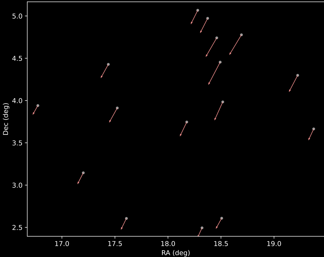
APOGEE DR17 Cluster 27 Proper Motion Vectors (n=16)
