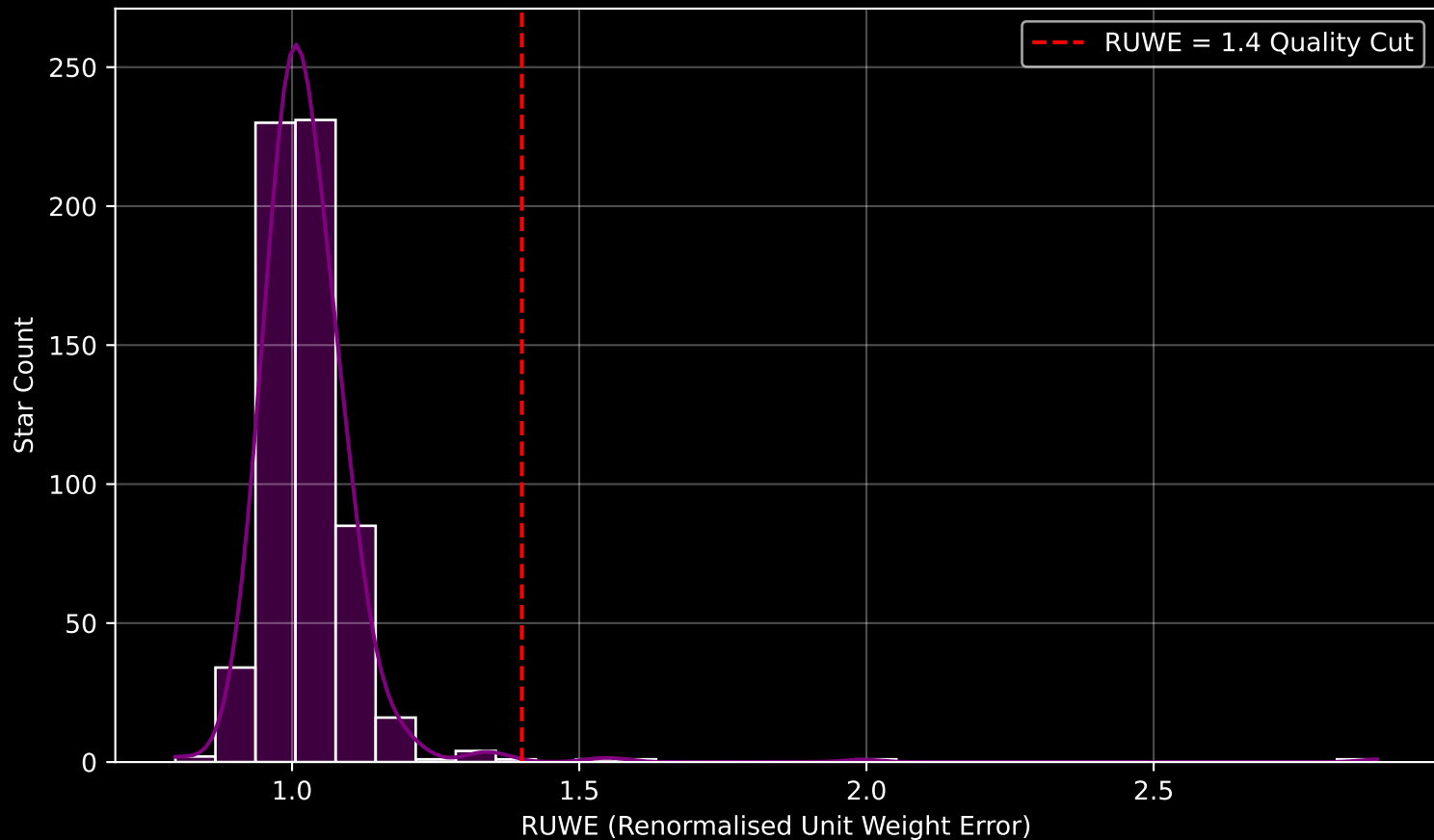
GAPOGEE DR17 Field [034+06] RUWE Distribution (n= 608)
