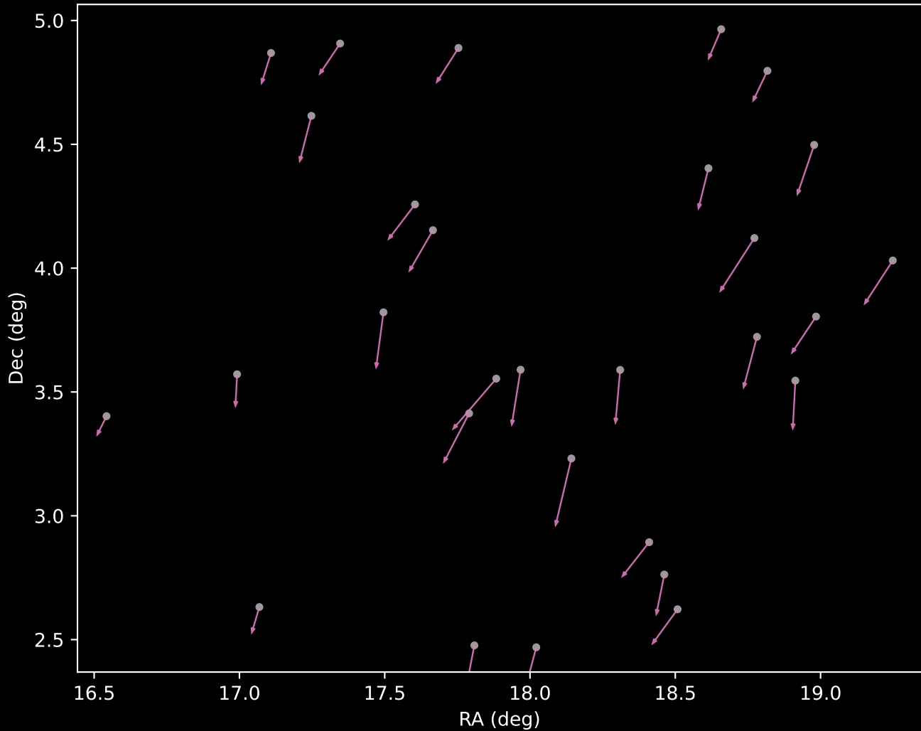
APOGEE DR17 Cluster 12 Proper Motion Vectors (n=29)
