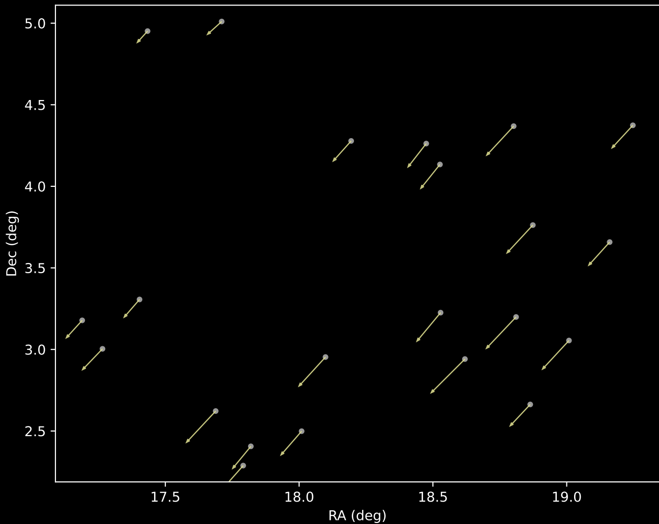
APOGEE DR17 Cluster 17 Proper Motion Vectors (n=22)
