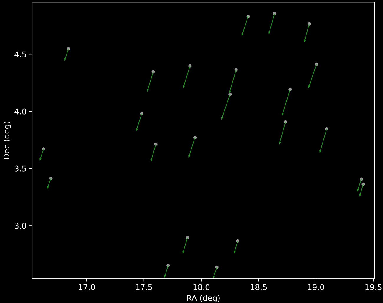
APOGEE DR17 Cluster 24 Proper Motion Vectors (n=23)
