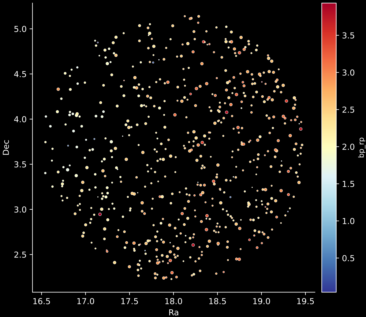
APOGEE DR17 Field: [034+06] Stars: 608
