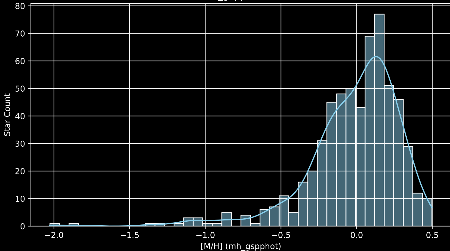
APOGEE DR17 Field: [034+06 [M/H] (mh_gspphot) (n= 599)
